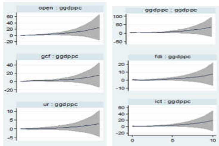
Impulse : Response — Orthogonalized IRF
